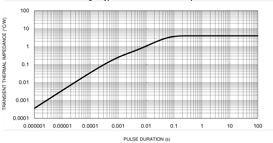
Fig.7 Typical Transient Thermal Impedance
